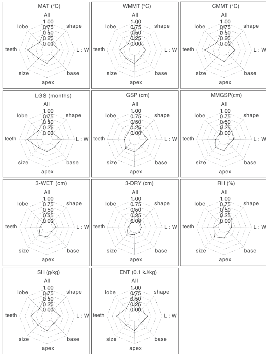
Fig. 4. Spider diagram showing the climatic signal coded by each feature class tested by the Climate Leaf Analysis with Neural Networks (CLANN). The radii represent the R-squared ( R^2 ) between the predicted and observed values for the complete physiognomic dataset (All), and other seven new datasets created by using just a single class of leaf characters from the physiognomic dataset each time. The physiognomic characters are grouped in seven classes: lobing, teeth, size, apex, base, length-to-width ratio (L:W), and shape. Abbreviations are as in Fig. 3.
