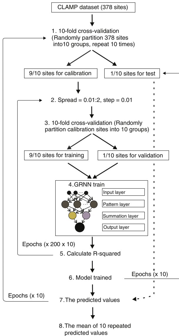
Fig. 1. Schematic illustration of the CLANN algorithm. (1) The entire dataset of 378 sites were randomly separated to 10 folds using 10-fold validation method in R. One of these folds was selected for test data and the other 9 folds for calibration data. This 10-fold validation was repeated 10 times. (2) Two hundred spreads (from 0.01 to 2, in steps of 0.01) were selected for model training. For each model the calibration was optimized with 20 \times 10 iterative cycles (epochs) (3) Next, calibration data were randomly separated to 10 folds using 10-fold validation method in R. One of these folds was selected for validation data and the other 9 folds for training data. (4) GRNN training. (5) The diagnostic values were calculated by comparing the predicted values and the real values. (6) The models were calibrated based on the optimal spread values. (7) Once the models were calibrated they were used to predict climate values for test data. The climate parameters of 378 sites were subsequently predicted using all the calibrated models for 10 iterative cycles (epochs). (8) The mean of all predicted climate parameters of 10 iterative cycles were calculated as a measure of the performance of the model.
