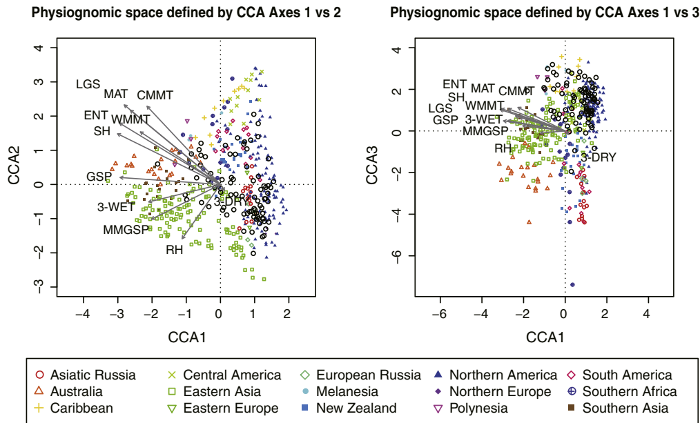
Fig. 5. Canonical correspondence analysis (CCA) showing that the 82 fossil sites used as CLANN test samples all fall within the physiognomic space defined by the modern dataset. CCA axes 1 vs 2 and CCA axes 1 vs 3 show the distribution of 82 North American Paleogene and Neogene fossil floras (black color open circles), within the cloud of modern sites (colored symbols) that define physiognomic space for the calibration dataset.
