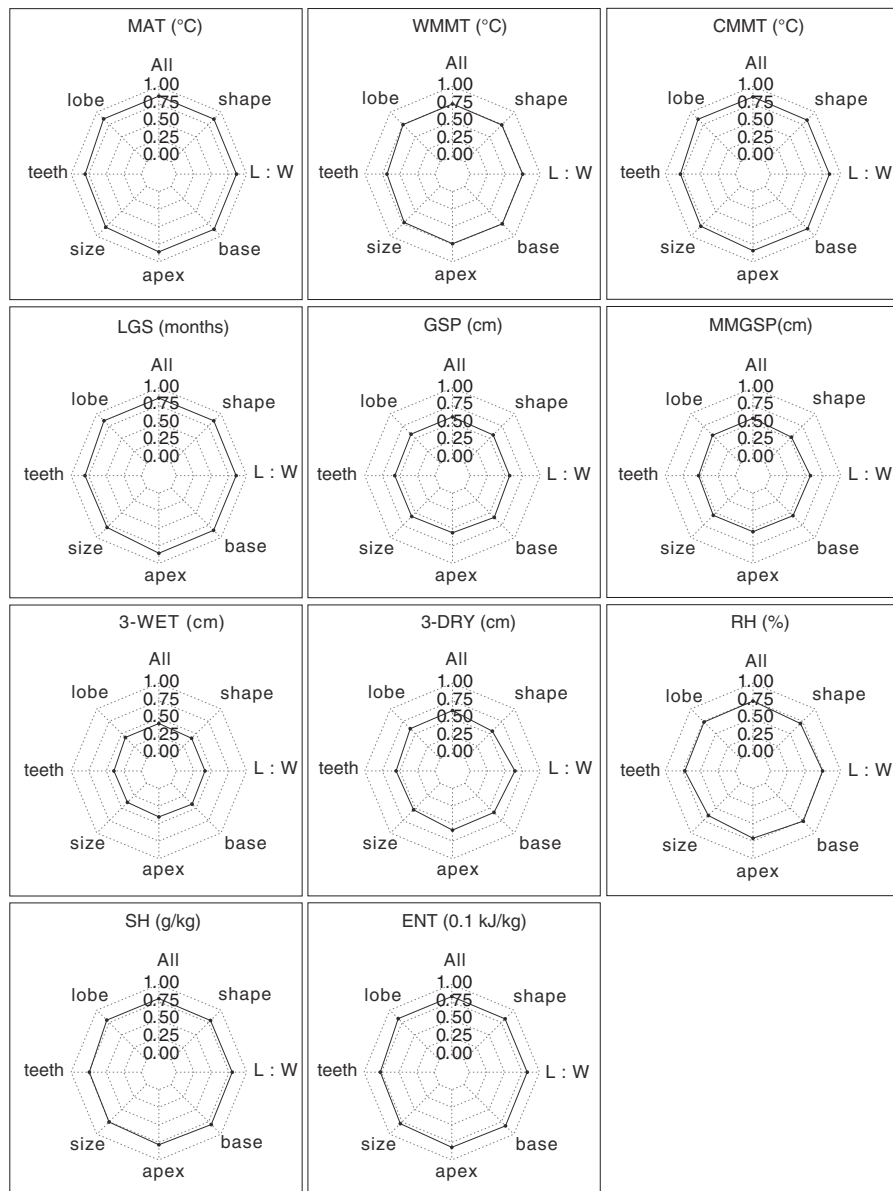
Fig. 3. Spider diagram showing the effect of character loss tested by the Climate Leaf Analysis with Neural Networks (CLANN). The radii represent the R^2 between the predicted and observed values for the complete physiognomic dataset (All), and other seven new datasets created by excluding a class of leaf characters from the physiognomic dataset each time. The physiognomic characters are grouped in seven classes: lobing, teeth, size, apex, base, length-to-width ratio (L:W), and shape. Abbreviations for the climate parameters: MAT, mean annual temperature; WMMT, mean temperature of the warmest month; CMMT, mean temperature of the coldest month; LGS, length of the growing season; GSP, growing season precipitation; MMGSP, mean monthly growing season precipitation; 3-WET, precipitation of the three consecutive wettest months; 3-DRY, precipitation of the three consecutive driest months; RH, annual mean relative humidity; SH, annual mean specific humidity; ENT, enthalpy.
