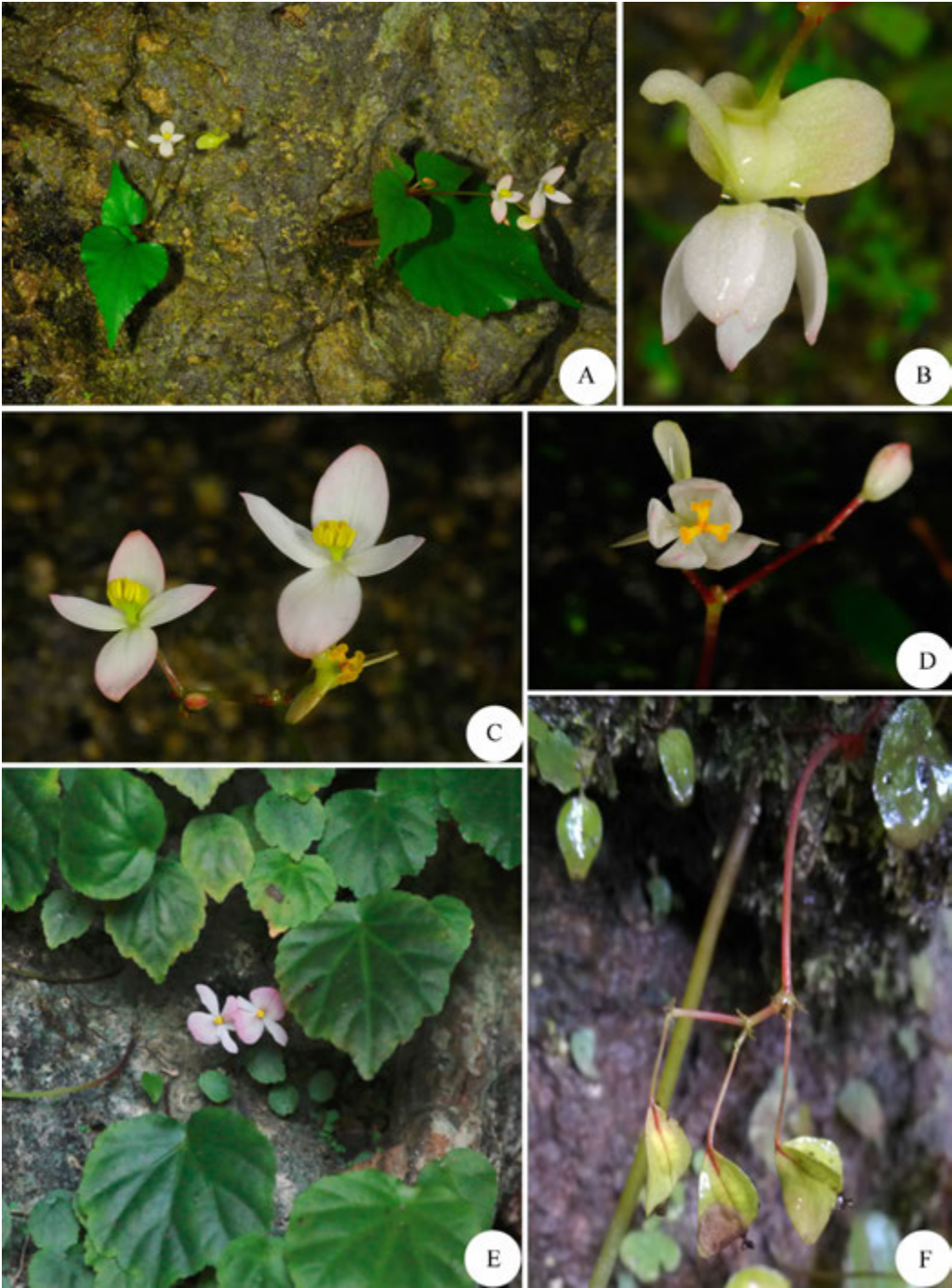
Fig. 1 Begonia demissa Craib and Begonia subperfoliata Parish ex Kurz A-D: Begonia demissa , A. Plants in their habitat; B. Side view on ovary; C. Male flowers; D. Female flowers. E-F: Begonia subperfoliata , E: Plants in their habitat; F: Fruits. ( A-D by SHUI Yu-min , E-F by LI Zhi-hong)
