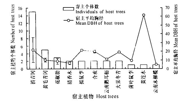
图 1 石林喀斯特山地森林中附生物宿主的个体数与平均胸径 Fig. 1 Number and mean DBH of host trees in forest at the Stone forest Karst Region
