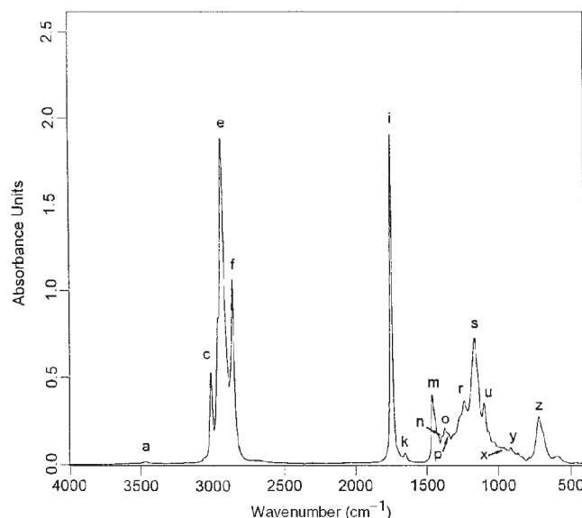
FIG. 1. FTIR spectrum of sachachi crude 1 (SIC1) oil.
