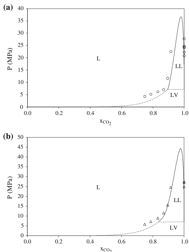
Fig. 4 Phase diagram for the binary system CO 2 + Sacha inchi seed oil at: (a) 303 K, and (b) 323 K. The parameters used to predict the phase equilibrium were k_{12} = 0.0039 and l_{12} = 0.3379
