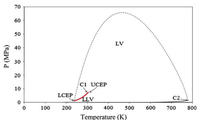
Fig. 5 Pressure versus temperature global phase diagram predicted for the binary system CO 2 + Sacha inchi seed oil. C1 CO 2 critical point, C2 Sacha inchi seed oil critical point, LV liquid-vapor equilibria, LLV liquid-liquid-vapor equilibria (thick line), UCEP upper critical end point, LCEP lower critical end point, critical points of the binary mixtures (broken lines), vapour pressure of pure CO 2 (dotted line), and vapour pressure of Sacha inchi seed oil (thin line)
