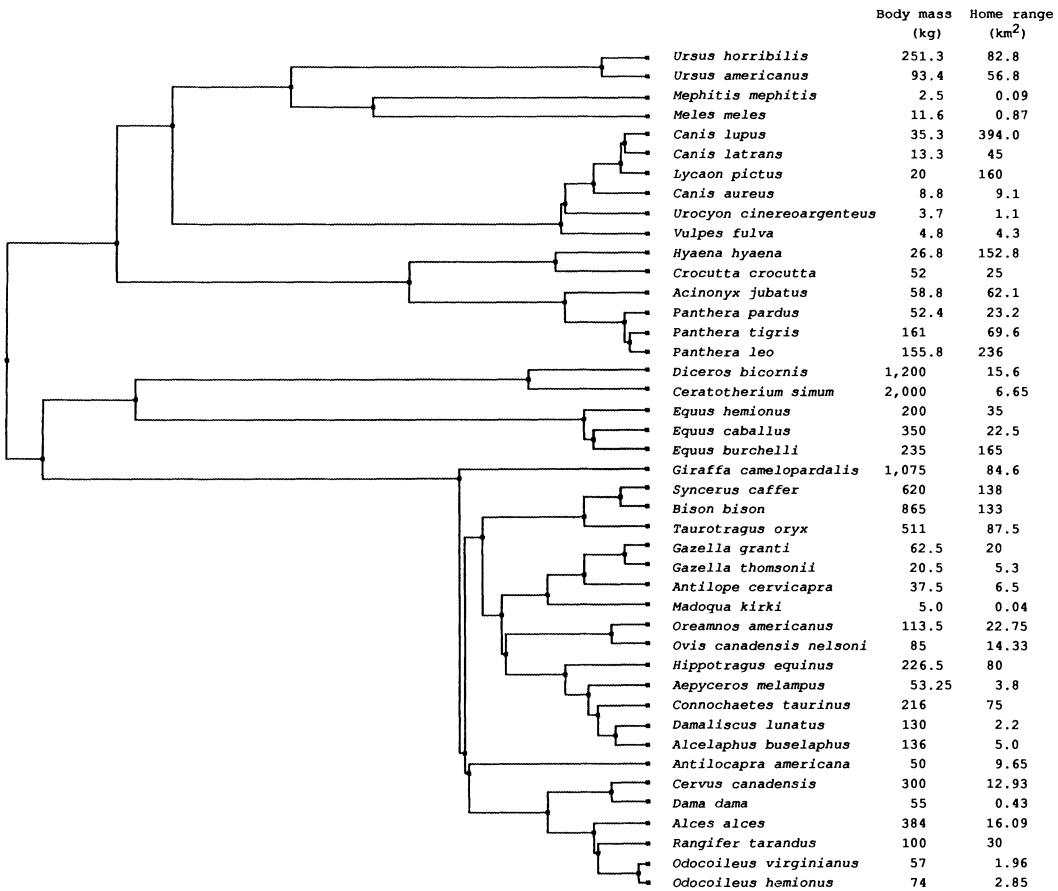
FIGURE 1. Phylogeny and data for body mass (kg) and home range area (km²) for 43 species of mammals (from Garland and Janis, 1992; Janis, in press). Branch lengths are in units of time, as estimated from first fossil appearances and from molecular clock information (sources in Garland and Janis, 1992). The shortest branch segment depicted is 0.5 million years; the basal split, between the Carnivora and the ungulates, is at 70 million years (complete specifications are available from the senior author). Although many other comparisons might be of interest, we note only the comparison of these two clades, which may generally be considered as predators and prey (Garland and Janis, 1992; Janis, in press).
