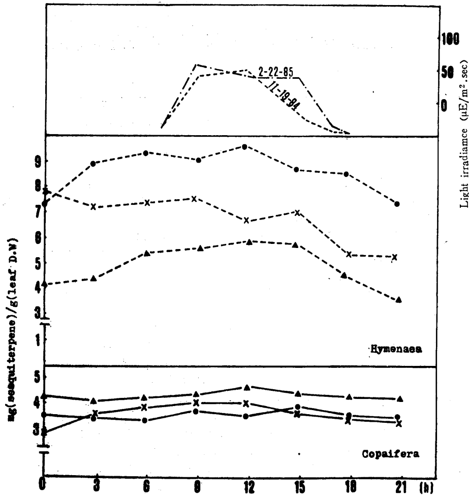
图1 H. courbaril 和 C. pubiflora C. officinalis 的倍半萜类化合物在三个季节的昼夜变化 Fig. 1 Diurnal variation of sesquiterpene yield for three dates (August 1984, November 1984 and February 1985) for H. courbaril and C. pubiflora and C. officinalis .
