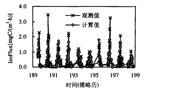
图 3 异戊二烯排放通量的观测值和计算值 Fig.3 The observed and calculated emission flux of isoprene
