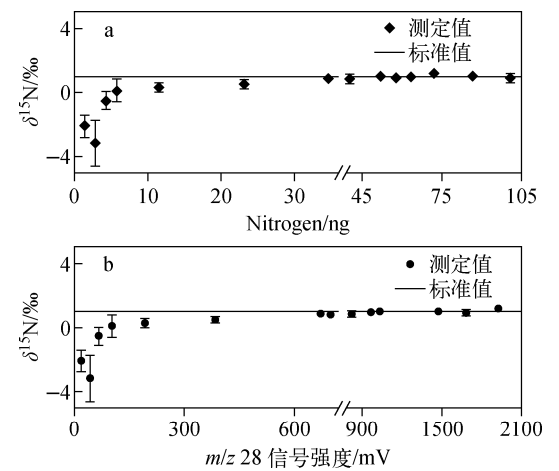
图2 GC-C-IRMS测定咖啡因 \delta^{15}\text{N} 的进样量(a)和信号强度(b)响应特征 Fig. 2 Response of GC-C-IRMS on caffeine \delta^{15}\text{N} measurement to sample size (a) and signal intensity (b)
