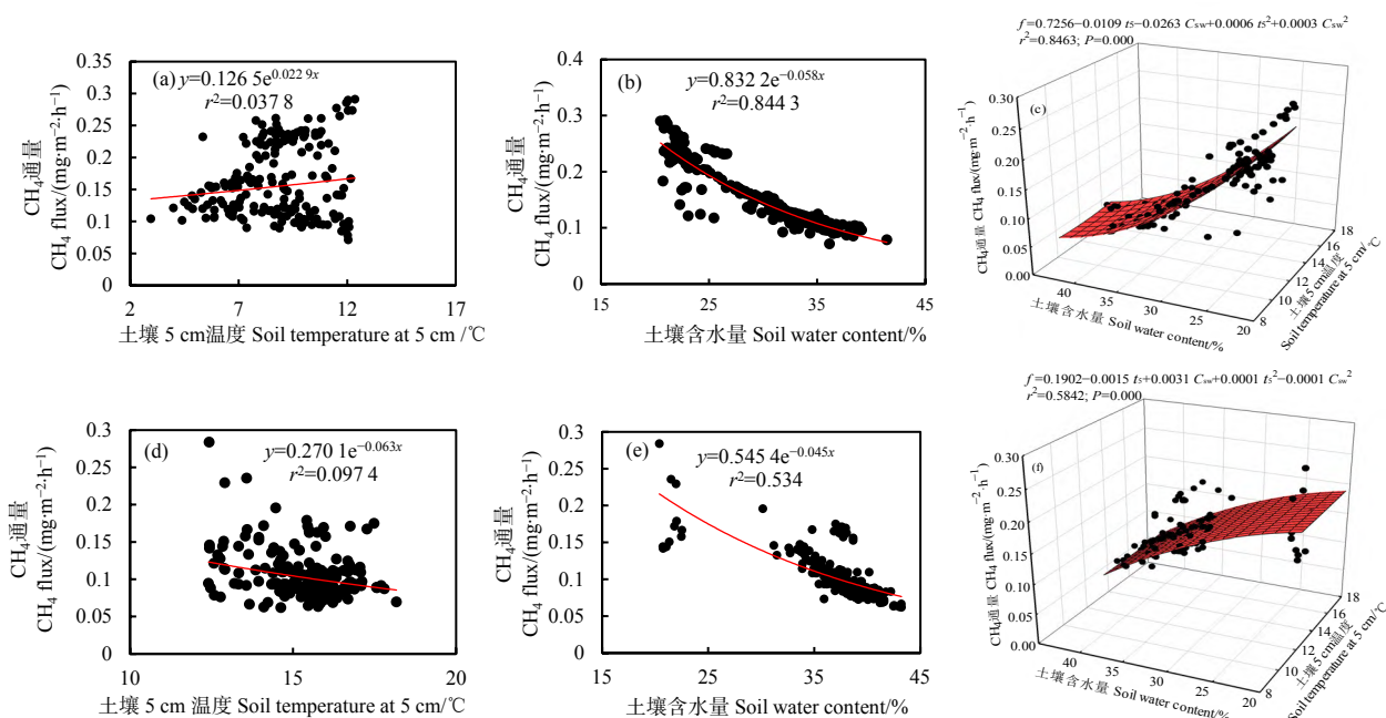
Figure 3 Exponential regression of temperature, soil water content with soil \text{CH}_4 flux and their two factors interaction
