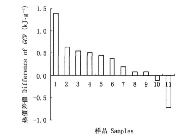
图 1 西双版纳热带季节雨林植物鲜叶和凋落叶的热值差值 Fig. 1 The difference of gross caloric value ( GCV ) between fresh leaves and leaf litters of plants in the tropical season rain forest in Xishuangbanna
