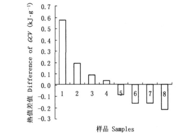
图 2 哀牢山中山湿性常绿阔叶林植物鲜叶与凋落叶热值的差值 Fig. 2 The difference of gross caloric value ( GCV ) between fresh leaves and leaf litters of plants in the mid-montane moist evergreen broad-leaved forest in Ailao Mountain
