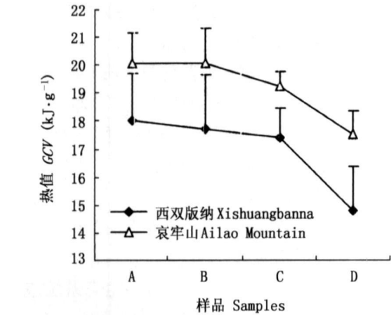
图3 西双版纳和哀牢山样品平均热值的比较(误差线表示标准误) Fig. 3 Comparison on average gross caloric value (GCV) of samples in Xishuangbanna and in Ailao Mountain (error bars represent standard error) A. 鲜叶 Fresh leaf B. 凋落叶 Leaf litter C. L 层 L layer D. F 层 F layer
