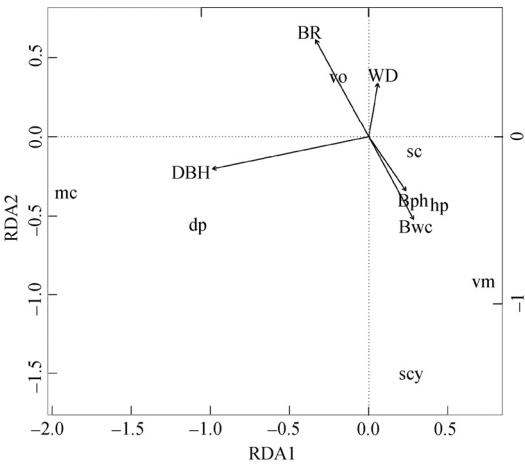
图 1 寄主植物的功能性状与桑寄生分布的冗余分析排序图。DBH: 胸径; WD: 木质密度; Bwc: 树皮含水量; BR: 树皮粗糙度; Bph: 树皮 pH。 Fig. 1 Redundancy analysis between host functional traits and the distribution of mistletoes on host. DBH: Diameter at breast height; WD: Wood density; Bwc: Bark water content; BR: Bark roughness; Bph: Bark pH.
